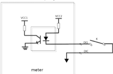
Digital input connection diagram
