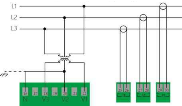
3PH4W (with PT) wiring diagram
