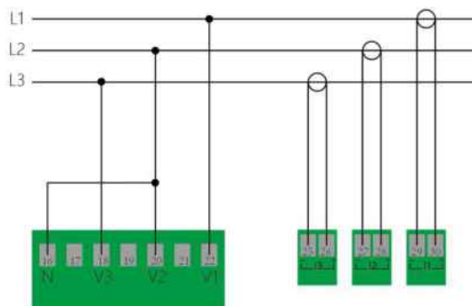
3PH3W (without PT) wiring diagram
