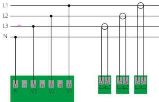
3PH4W (without PT) wiring diagram
