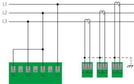
3PH3W (without PT) wiring diagram
